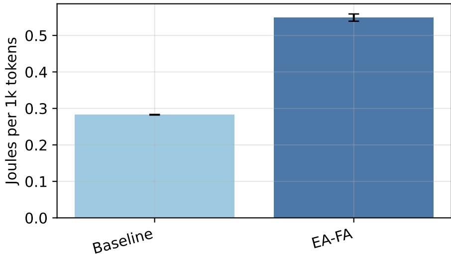
Energy-to-solution (lower is better)
