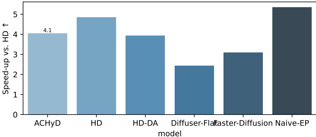
Experiment 2 - Module Ablations (synthetic)
