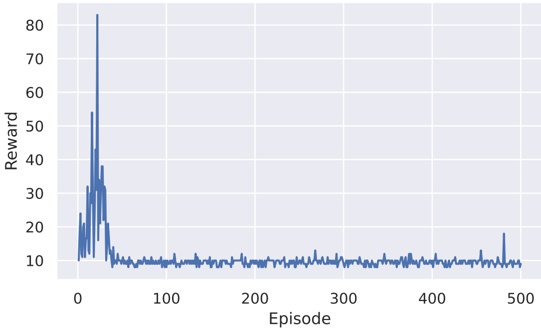
Training curve - CartPole (REINFORCE)
