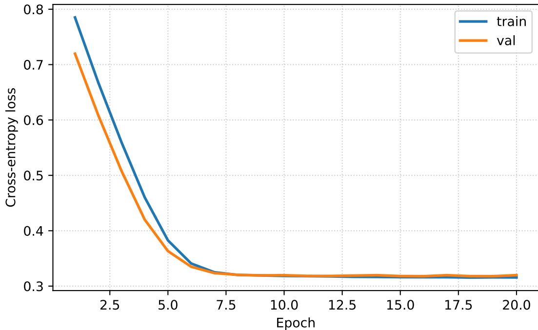
Training curves - SimpleNet
