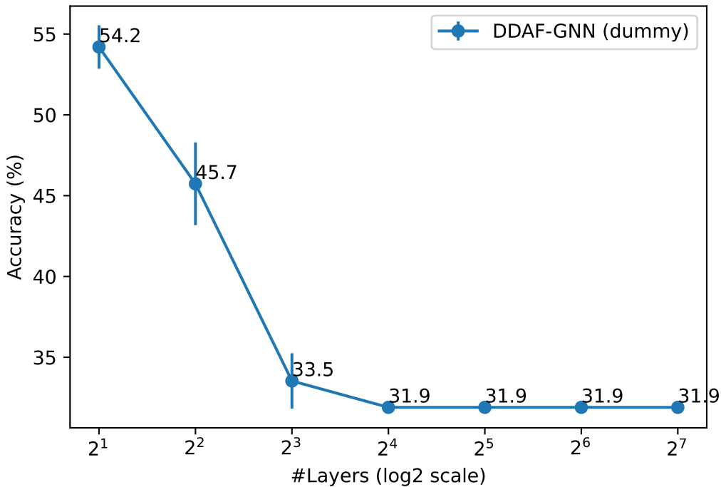
Cora - Depth vs Accuracy
