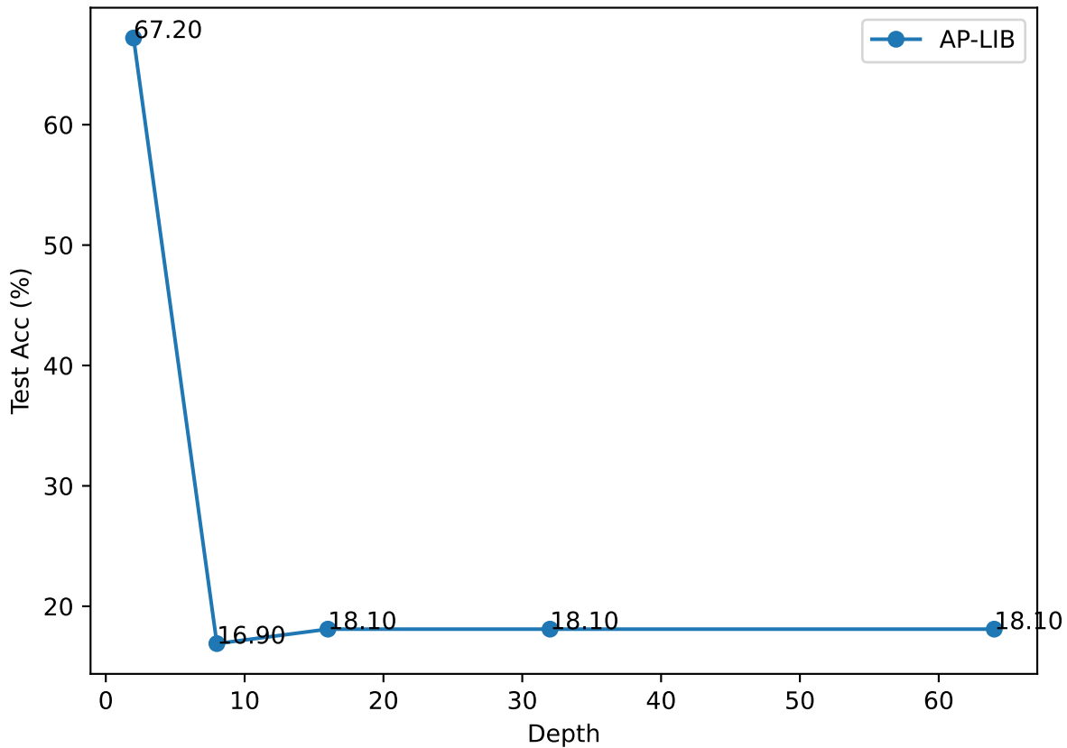
Citeseer - accuracy vs depth
