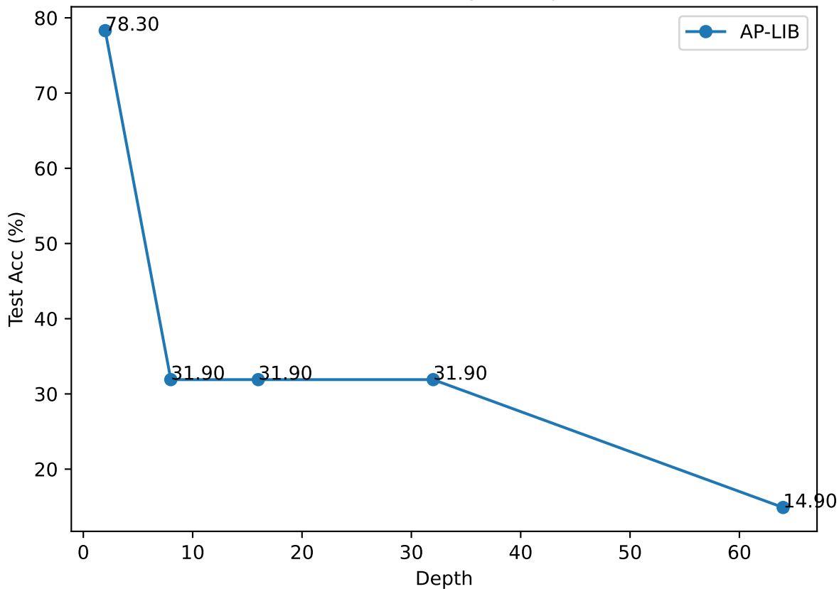
Cora - accuracy vs depth
