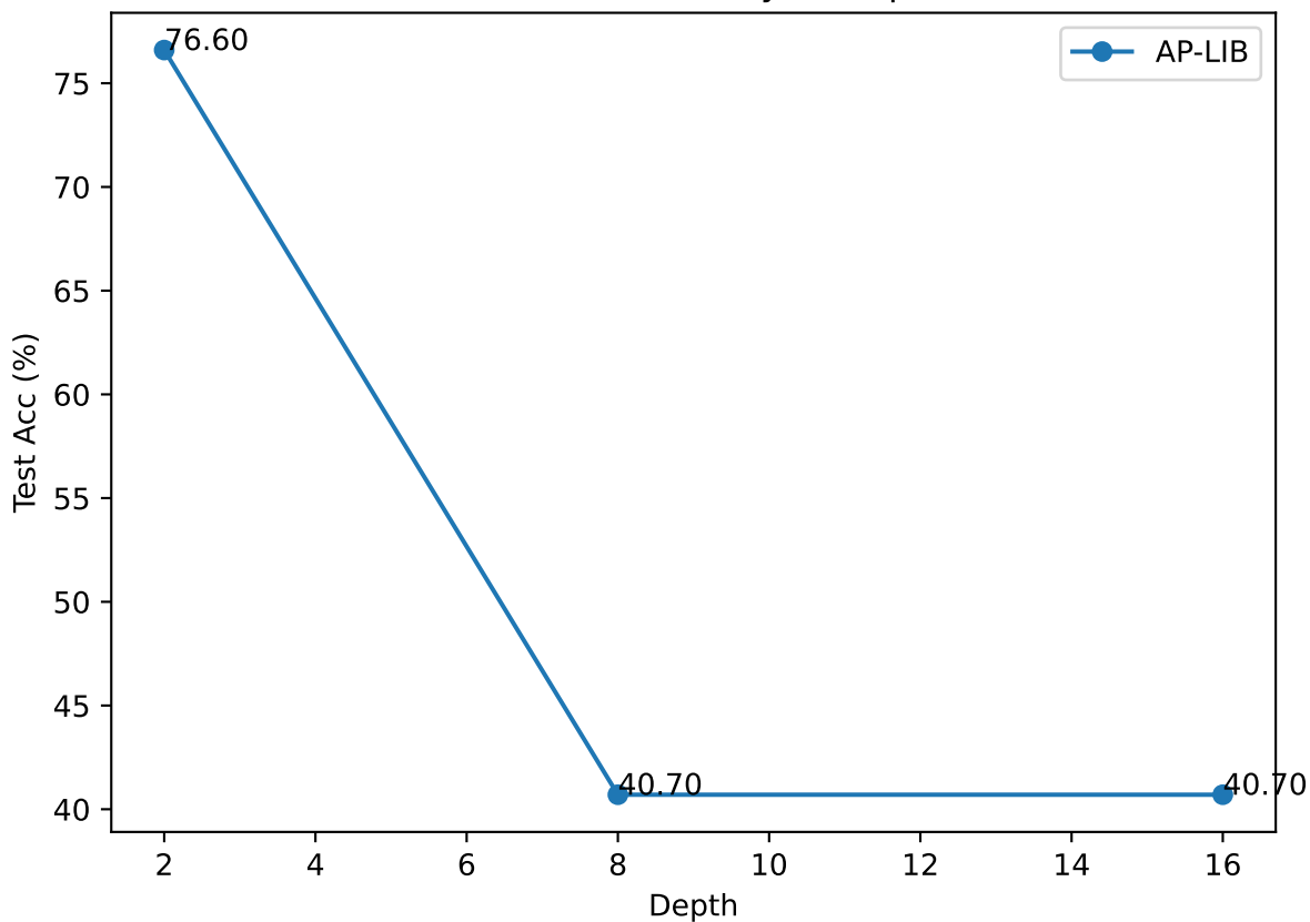
PubMed - accuracy vs depth
