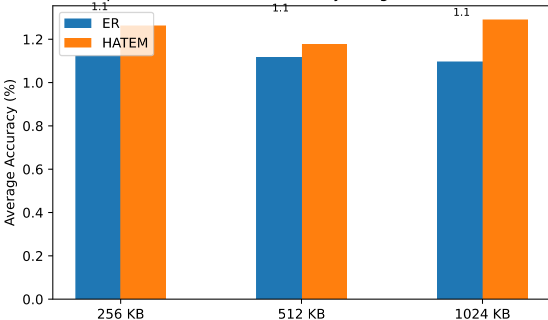
Experiment-1: AACC vs Memory Budget on CIFAR-100
