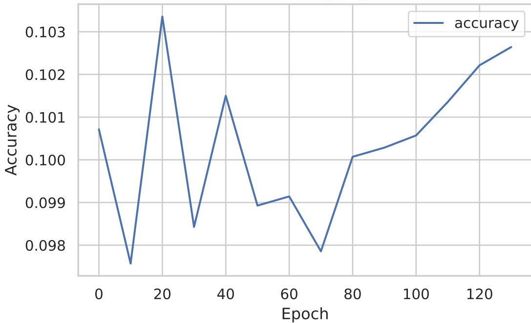
Accuracy - apd_gcn_exp1
