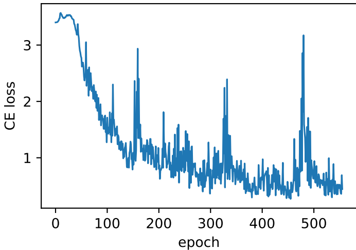
Val-loss Path-of-Cliques depth=8
