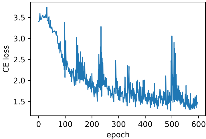
Val-loss Ring-of-Cliques depth=16
