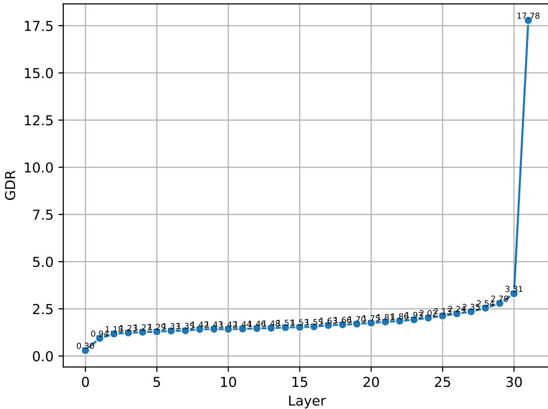
GDR Mixture PairNorm
