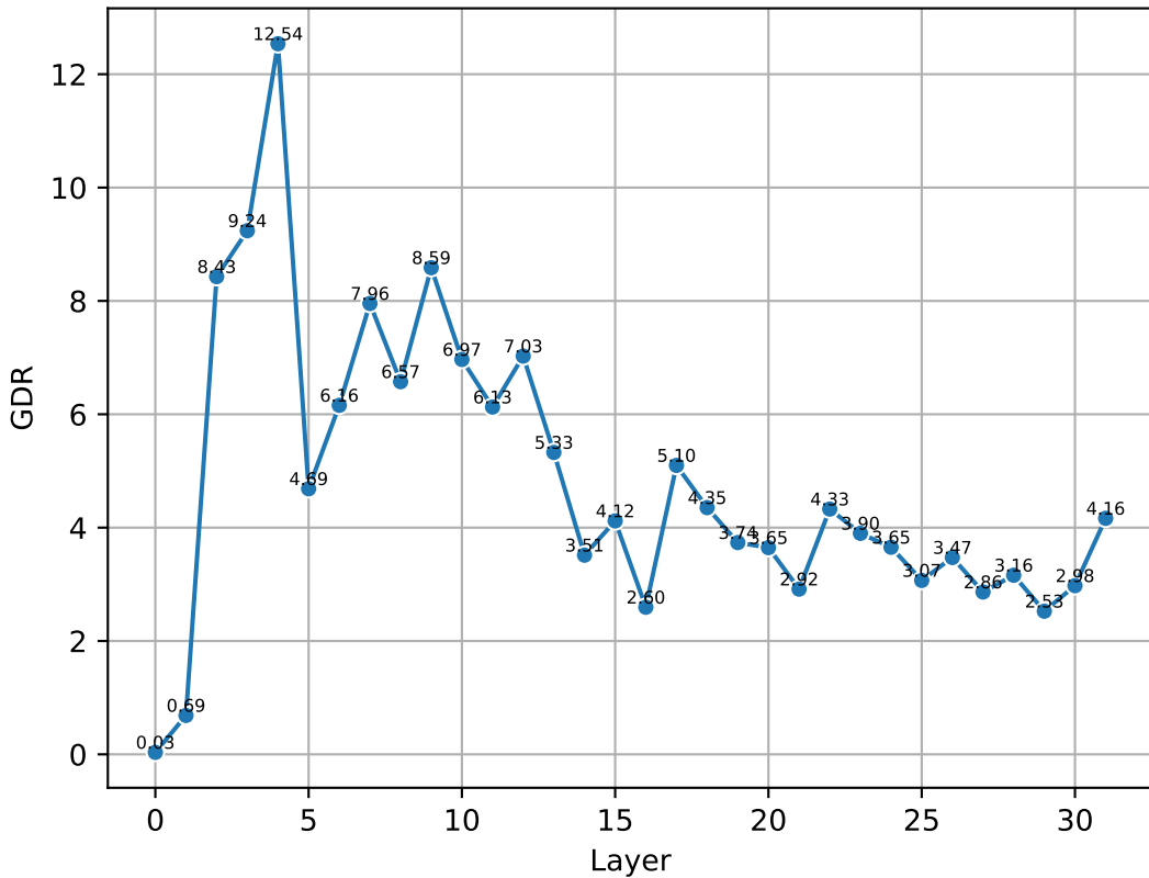
GDR Path-of-Cliques CurvAMP
