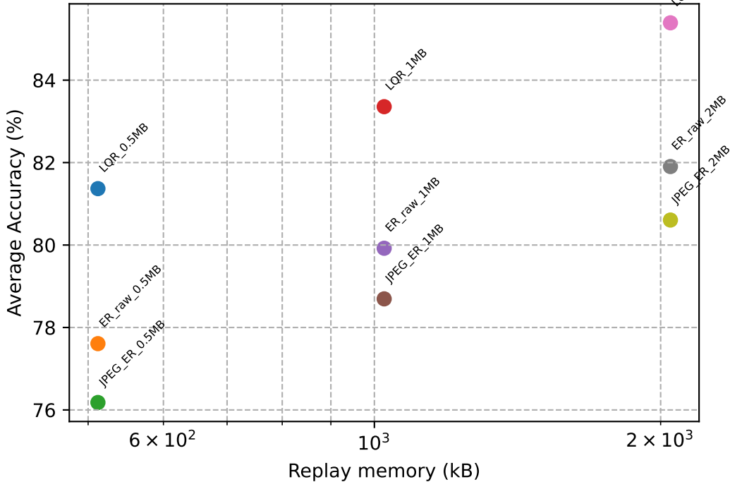
Memory-Accuracy Pareto (Split CIFAR-100)
