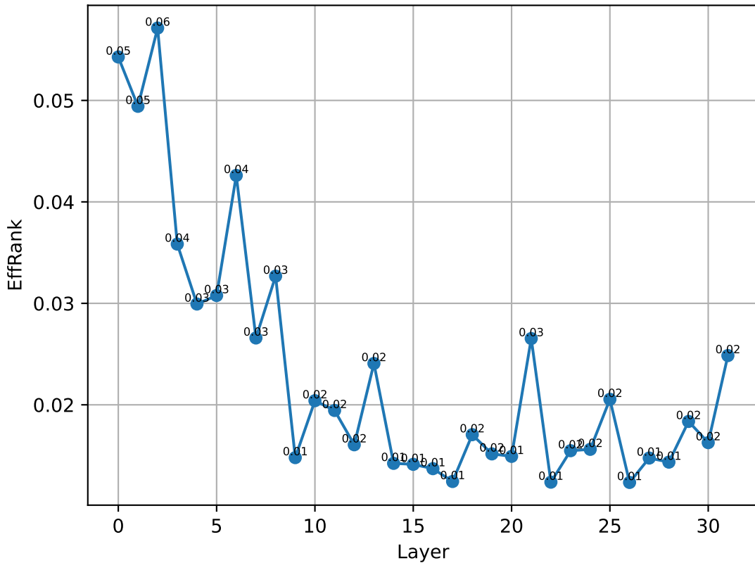
EffRank - Ring-of-Cliques
