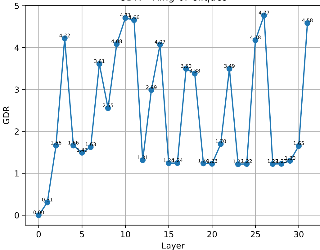
GDR - Ring-of-Cliques
