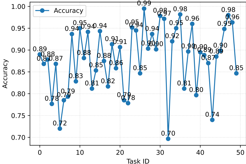
EXP1 - Accuracy over Tasks
