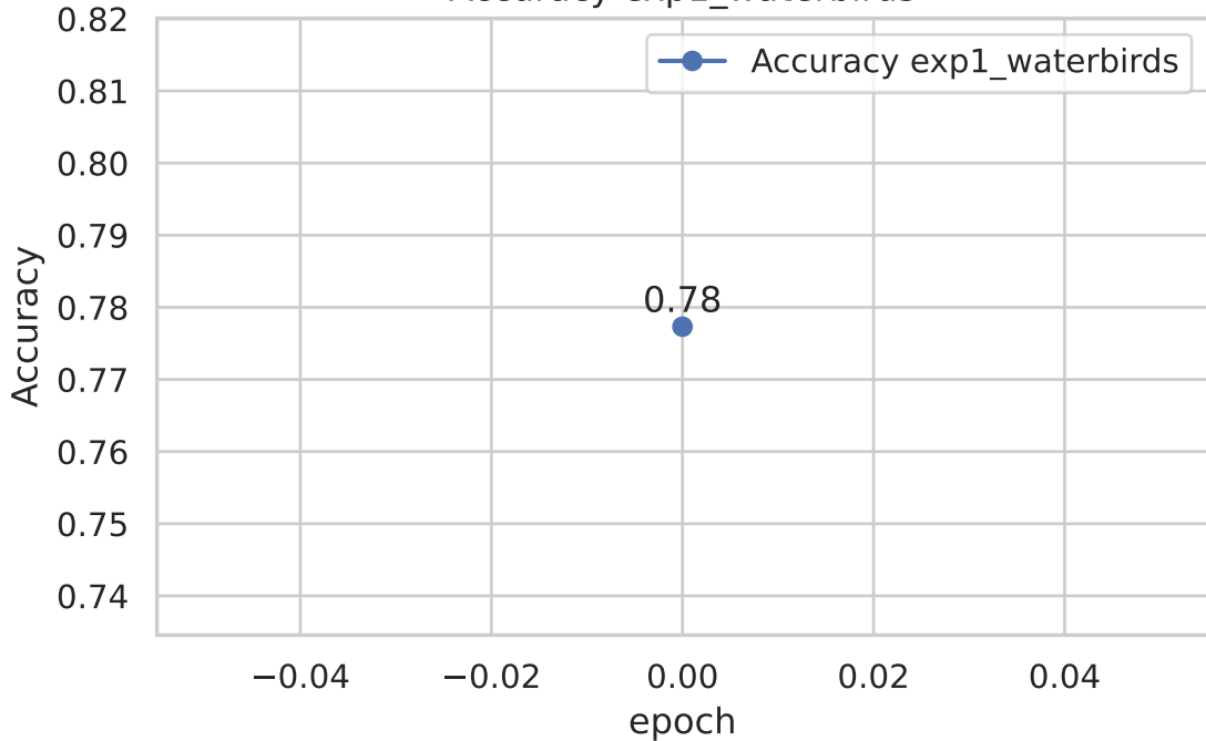
Accuracy exp1_waterbirds
