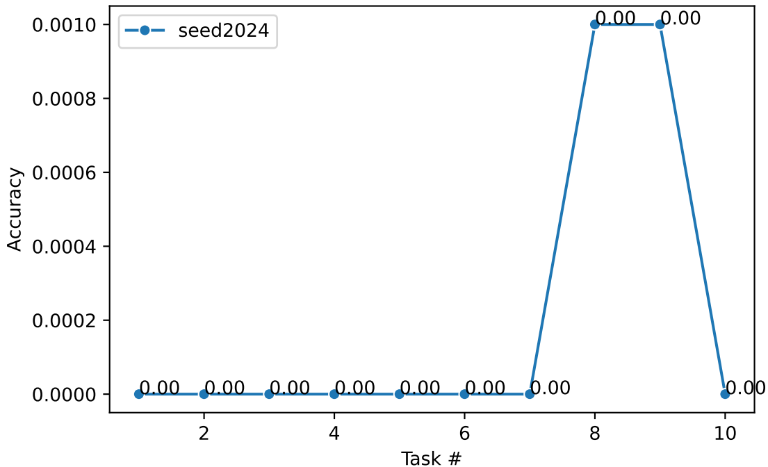
Accuracy - B=0.25 MB seed=2024
