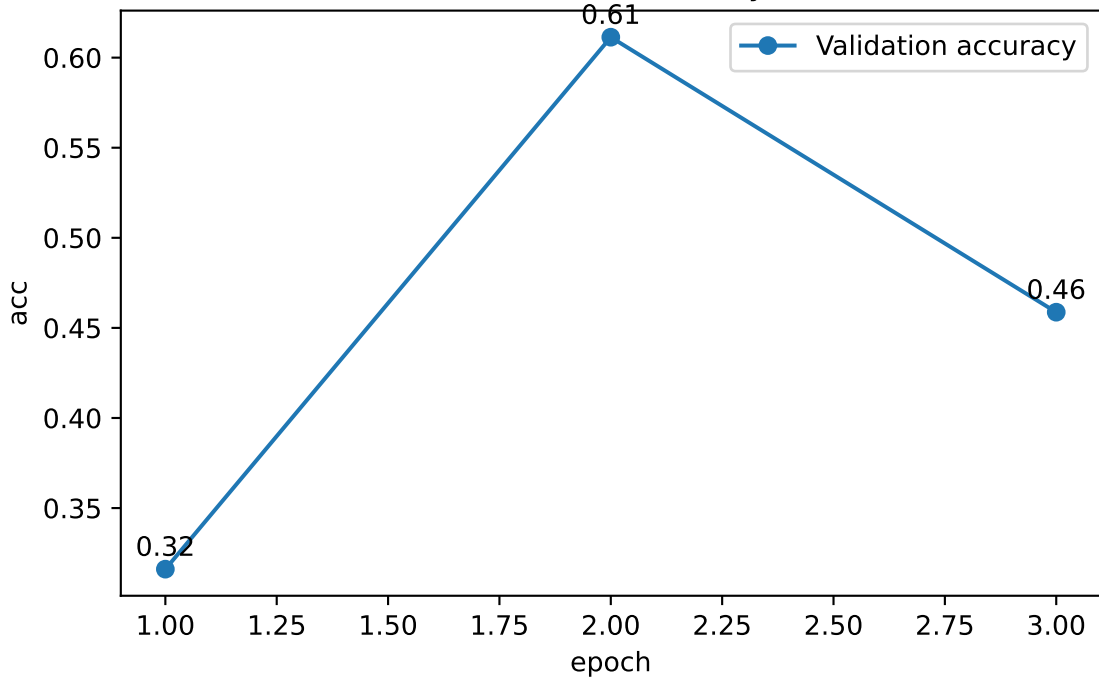
Validation accuracy
