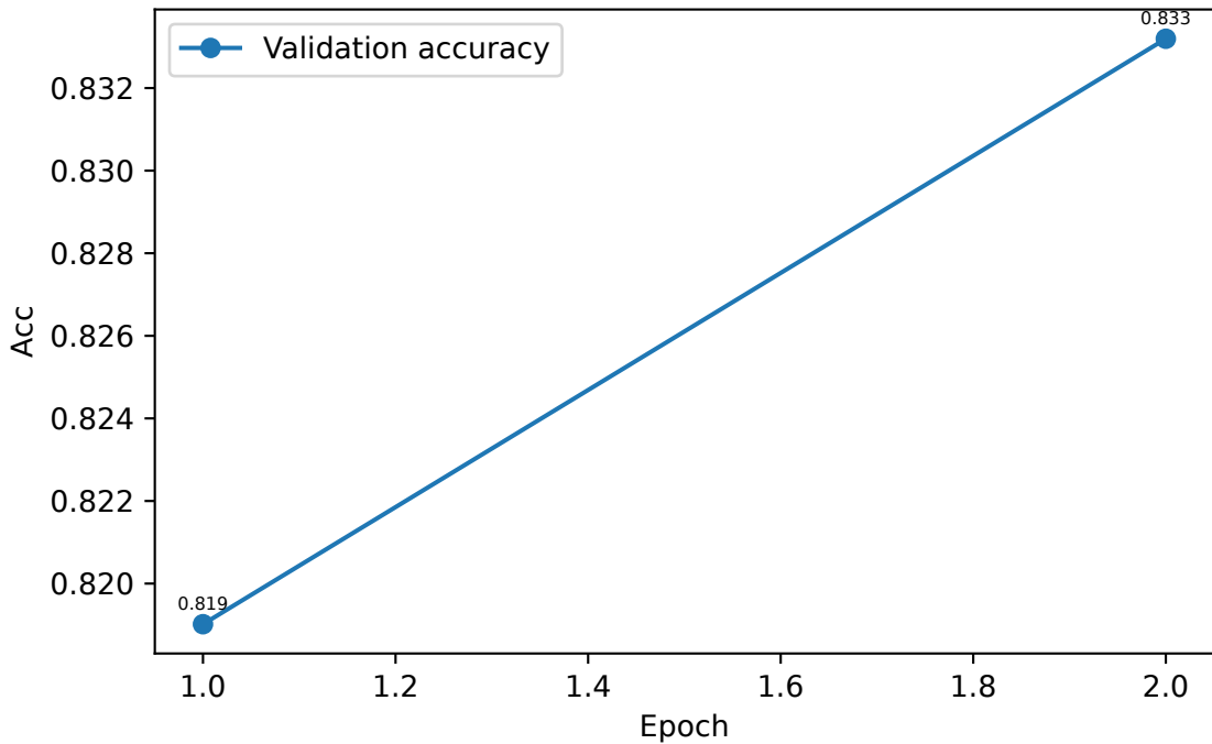
Validation accuracy
