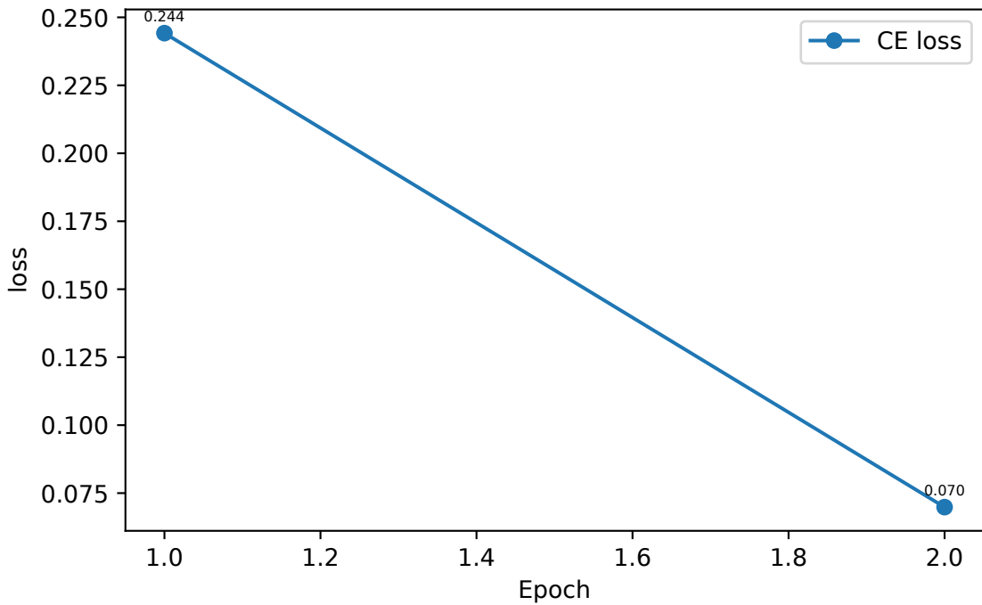
CE loss
