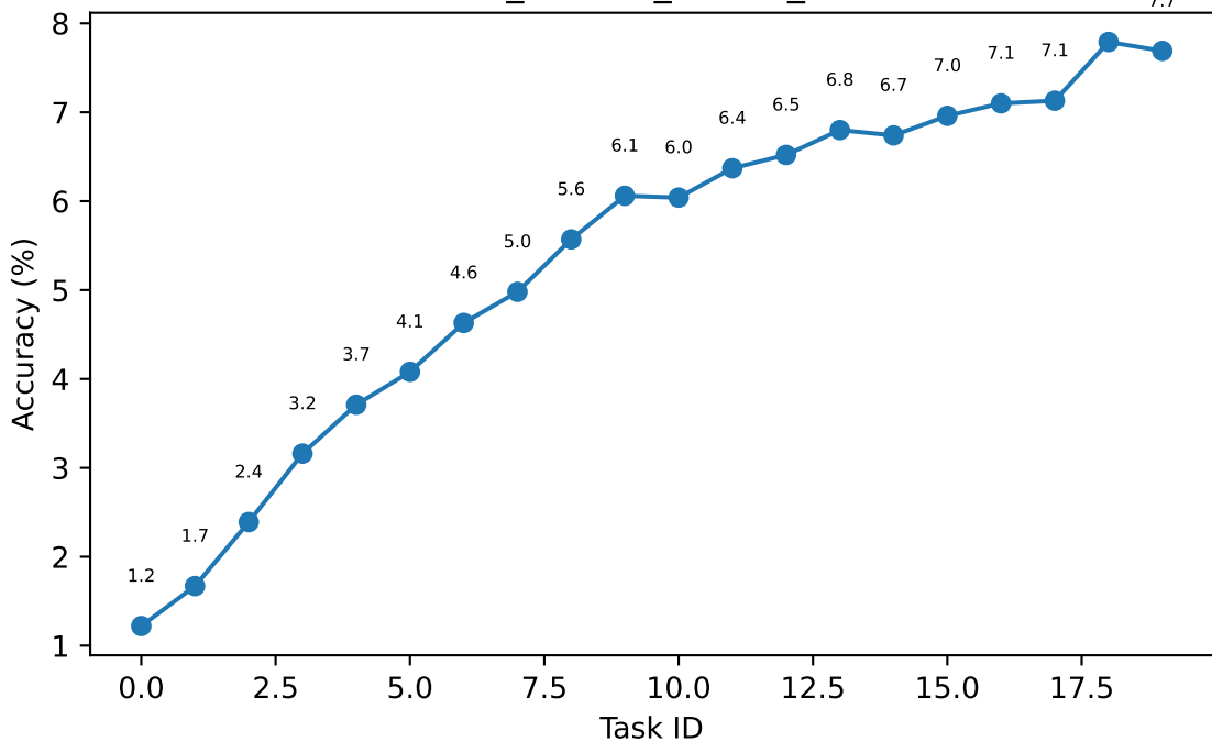
cifar100_coreset_bilevel_1024KB
