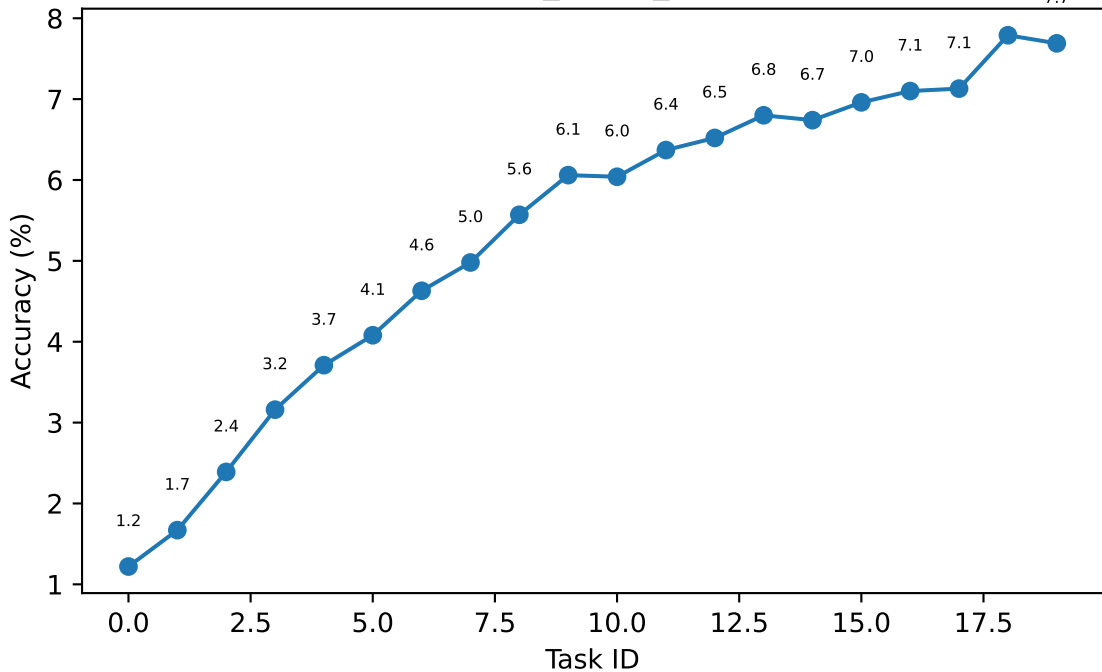
cifar100_derpp_500KB
