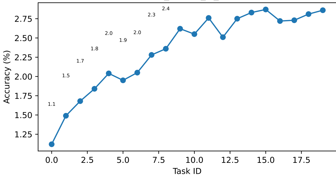
cifar100_sketch_cl_500KB
