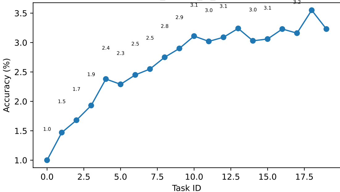
cifar100_sketch_cl_5120KB
