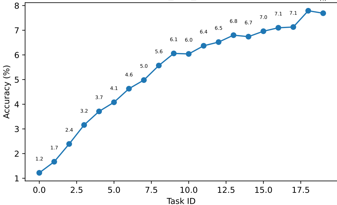
cifar100_ucb_5120KB
