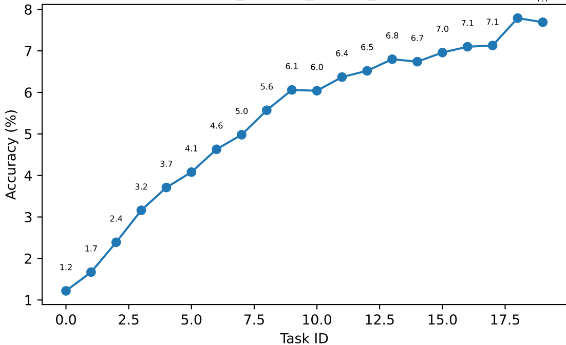
cifar100_coresets_bilevel_5120KB
