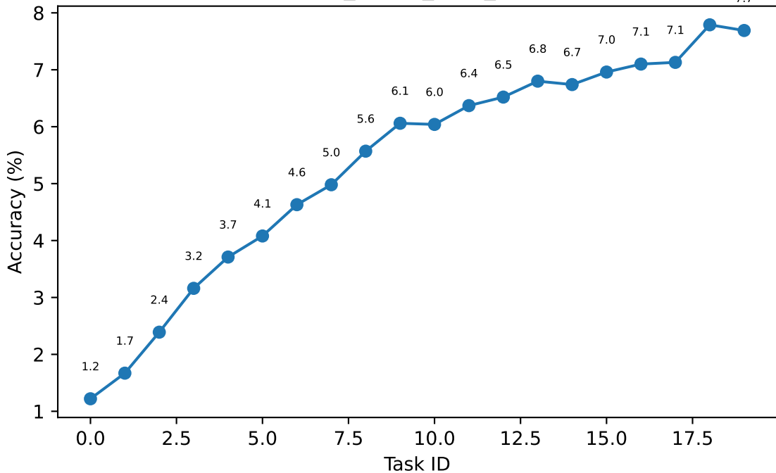
cifar100_sparcl_dgm_5120KB
