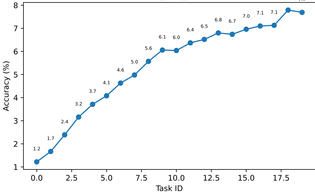
cifar100_ucb_500KB
