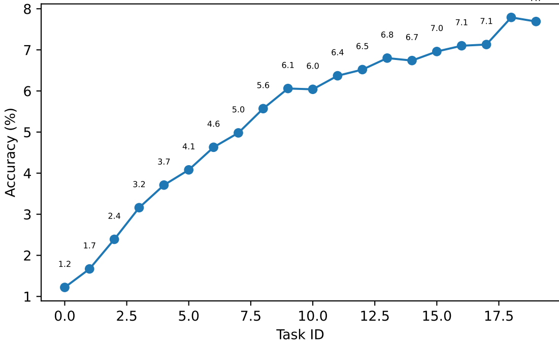
cifar100_uniform64_5120KB
