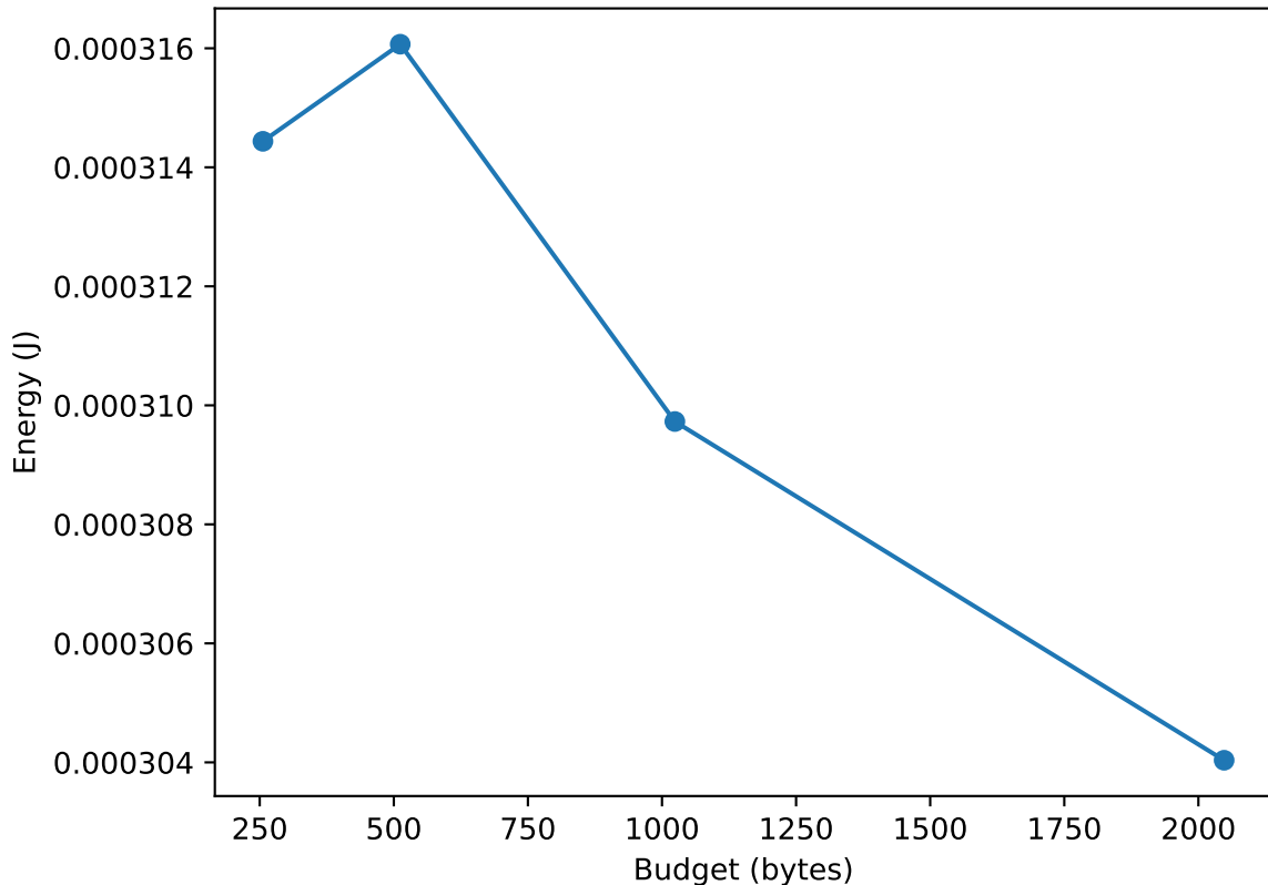
Experiment-3 Energy vs Memory Budget
