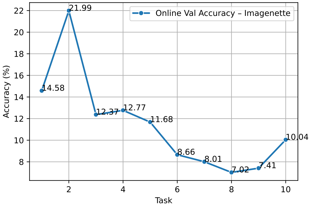
Online Val Accuracy - Imagenette
