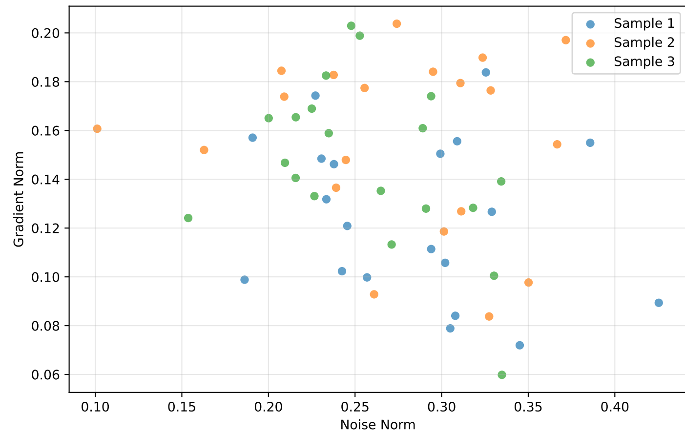
Noise vs Gradient Norms
