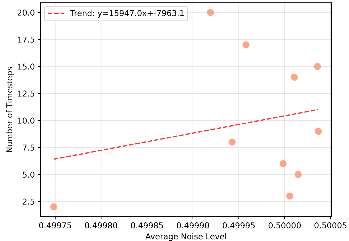
Noise Level vs Sample Complexity
