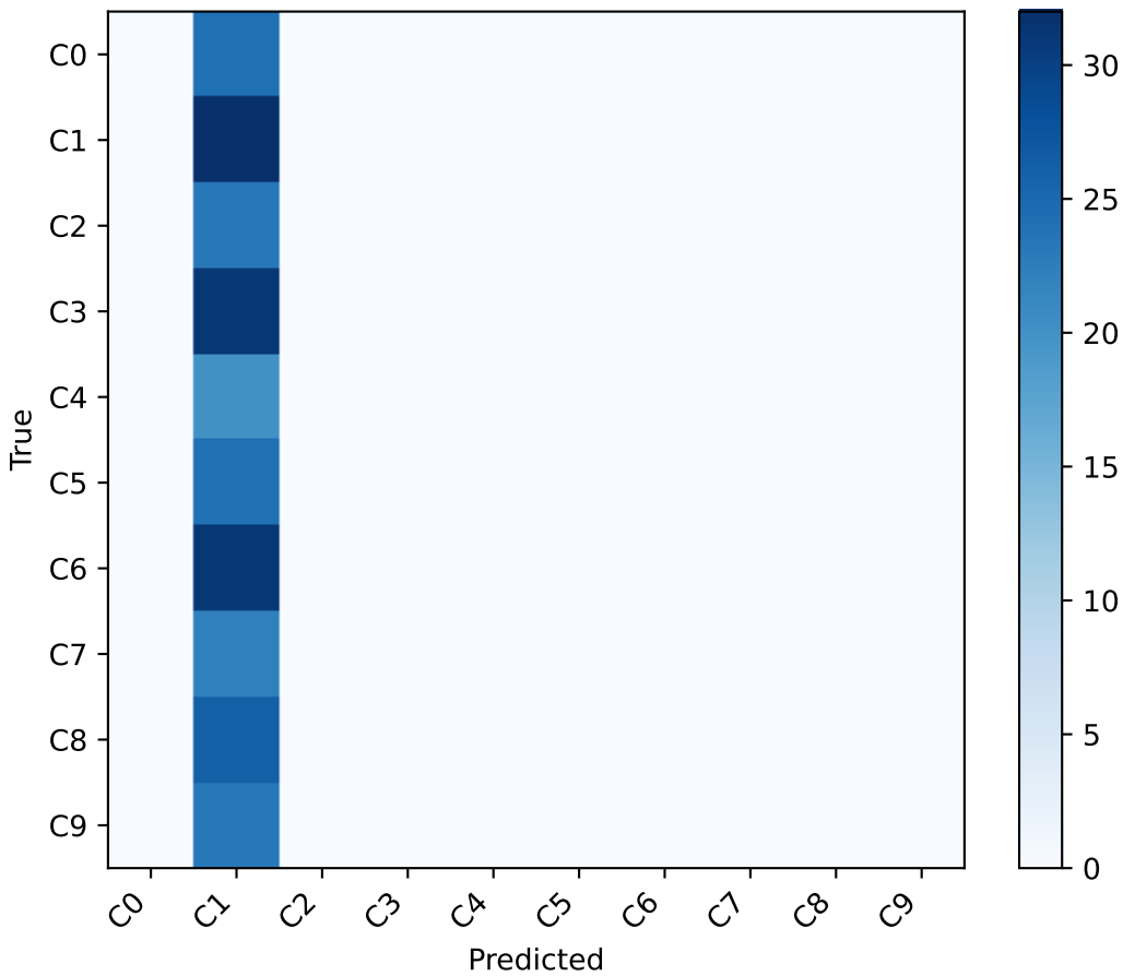
Confusion Matrix (IAQ-4)
