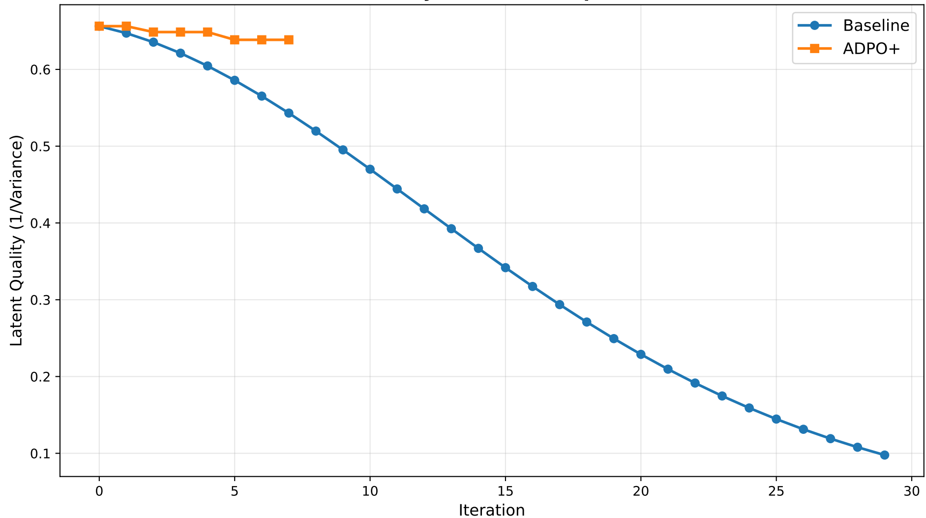
Latent Quality Evolution - Experiment 1
