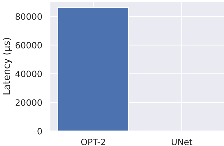
Embedding latency
