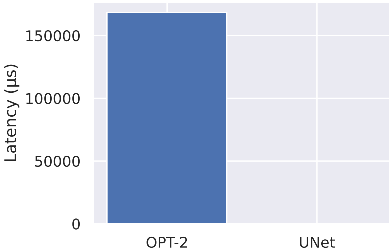
Embedding latency
