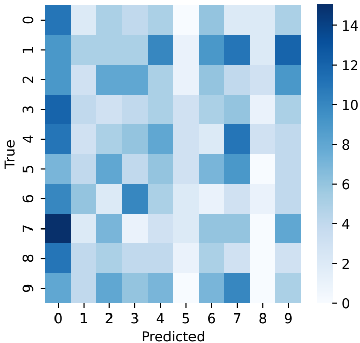
ASRIN Confusion Matrix (MNIST)
