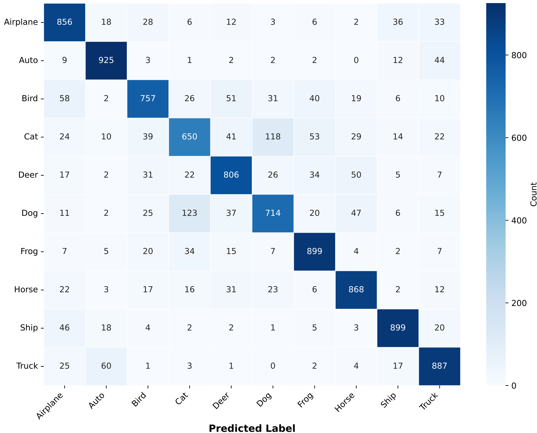
Confusion Matrix - proposed-resnet18-cifar10
