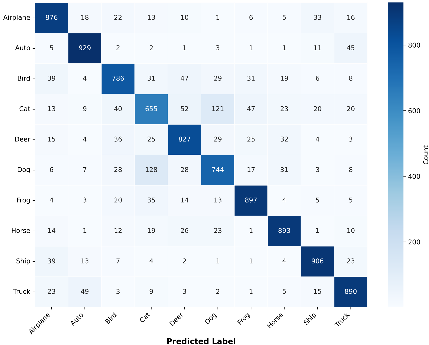
Confusion Matrix - comparative-1-resnet18-cifar10
