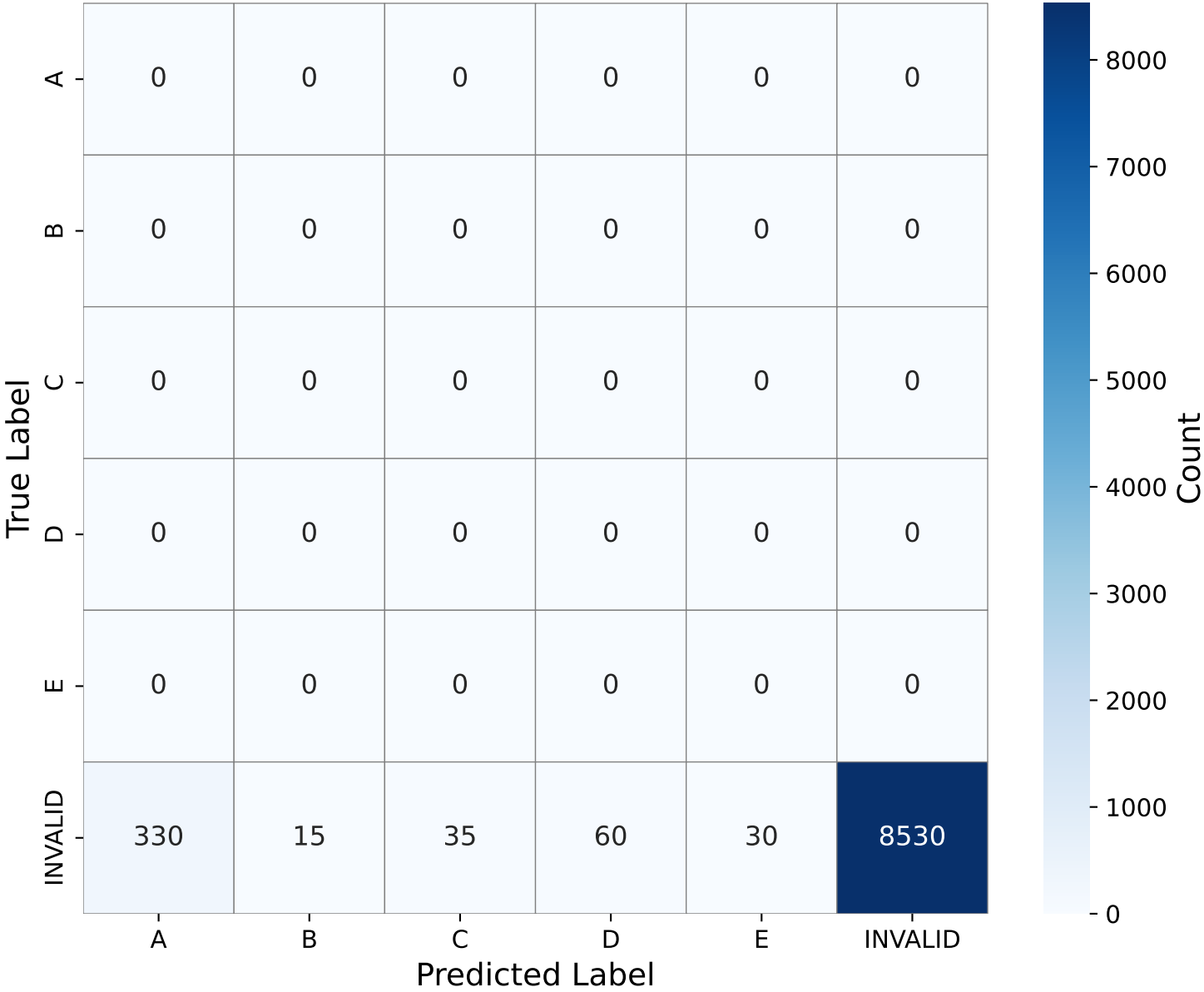
Confusion Matrix
