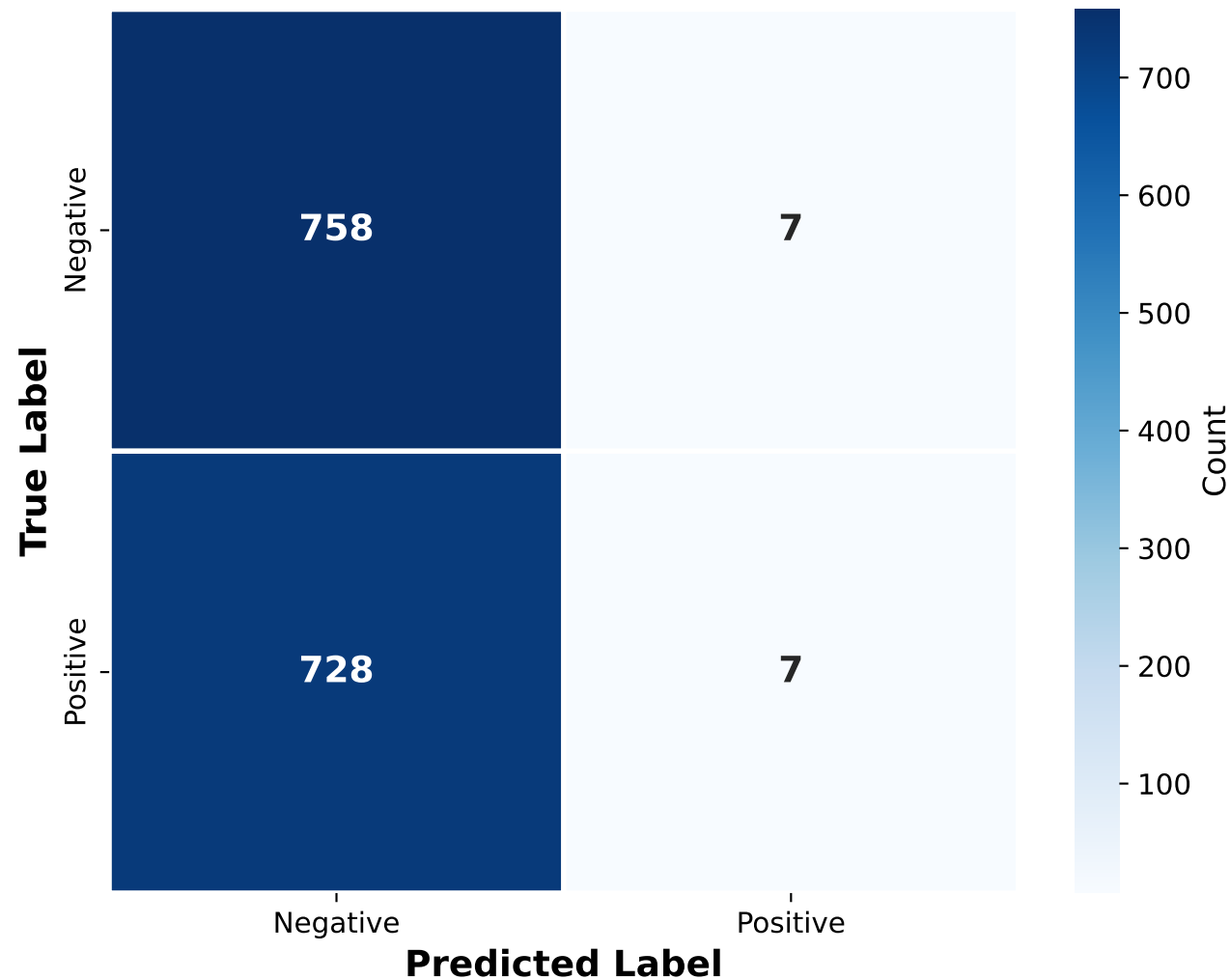
Confusion Matrix - SST2
