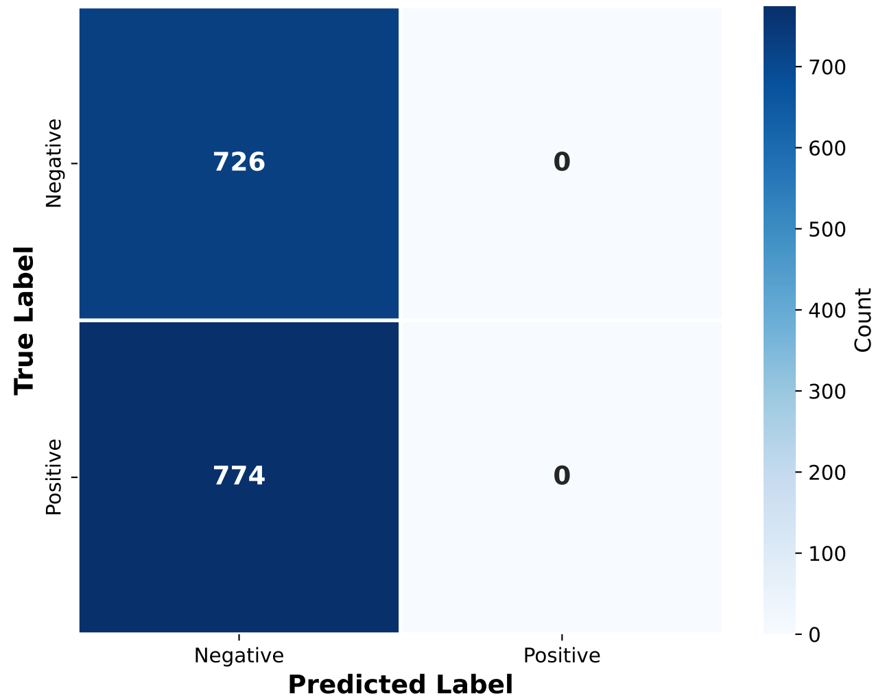
Confusion Matrix - IMDB
