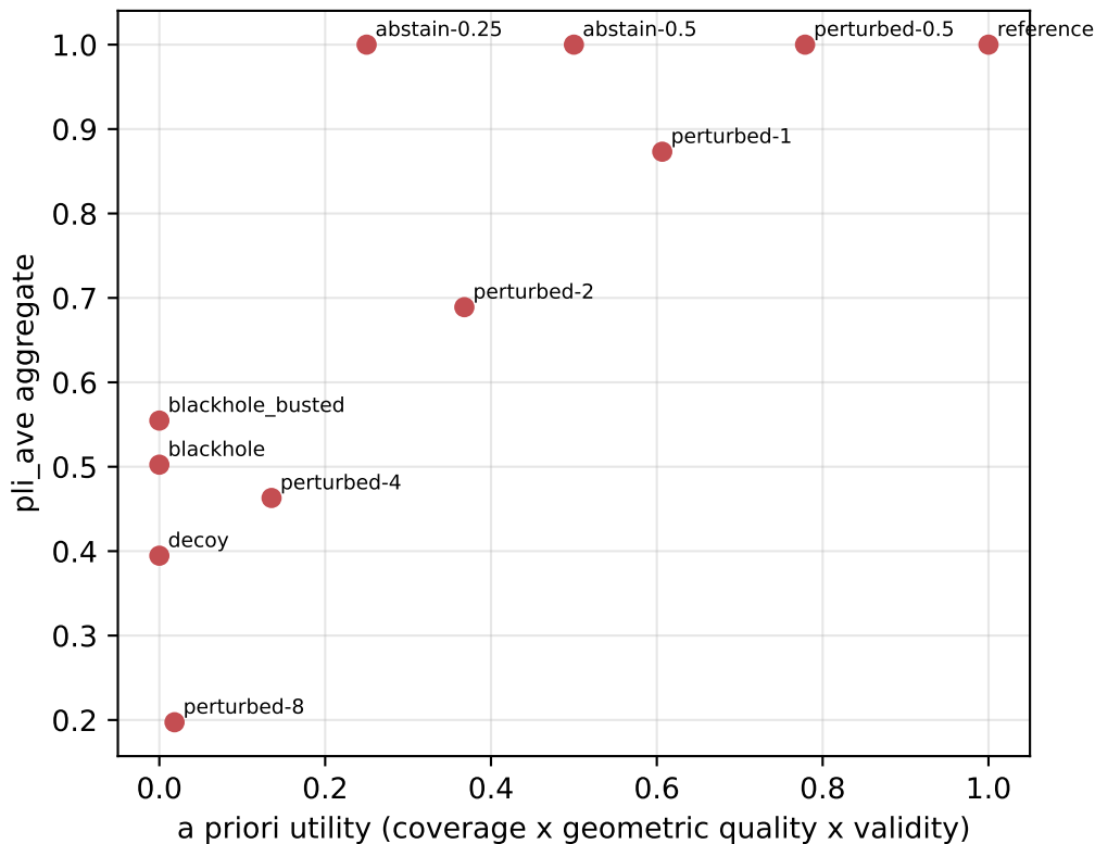
comparative-1-plinder-mlsb: rank fidelity \rho=0.775
