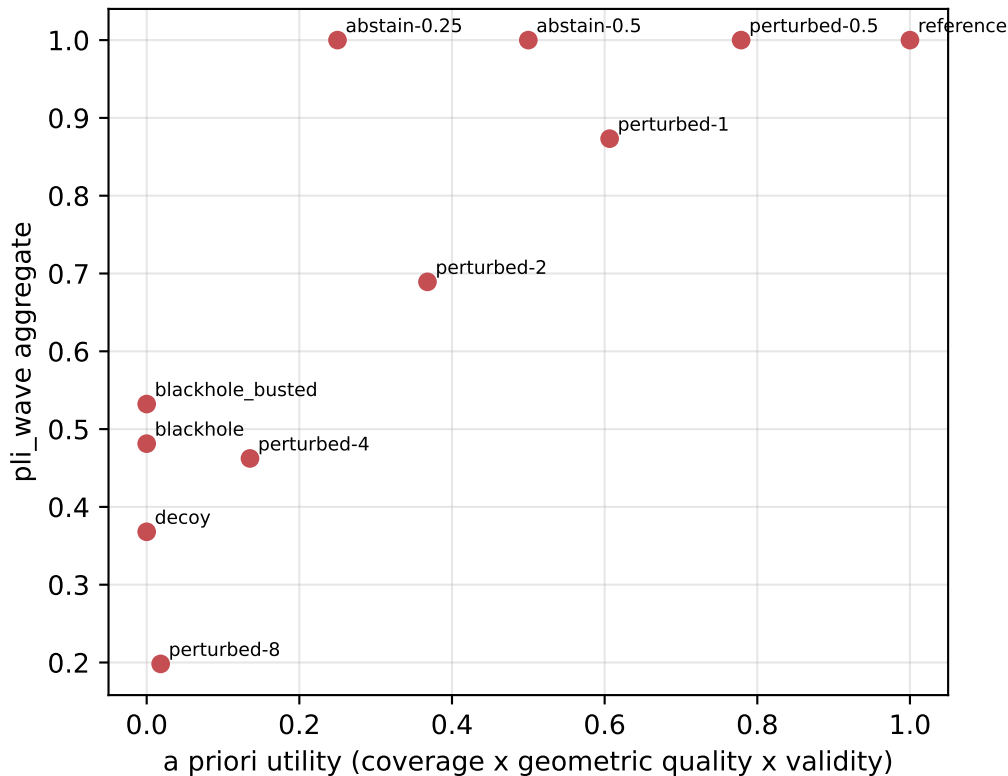
comparative-2-plinder-mlsb: rank fidelity \rho=0.775
