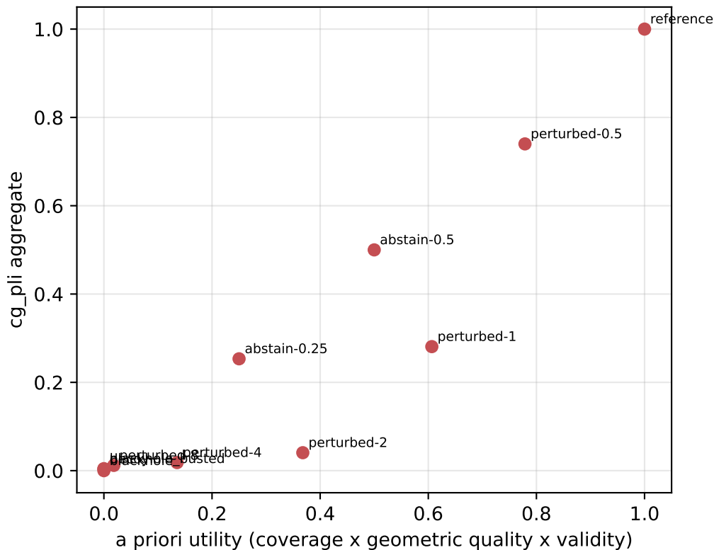
proposed-plinder-mlsb: rank fidelity \rho=0.973
