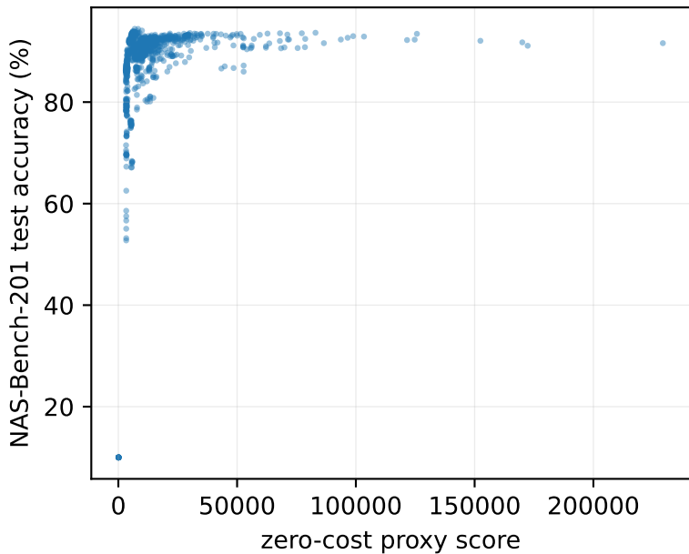
comparative-3-snip-cifar10
