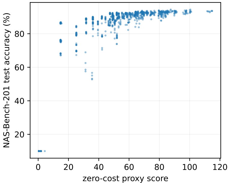
comparative-6-synflow-randinput
